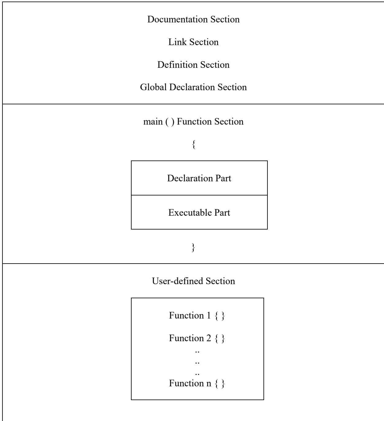
Image 1: Structure of programs written in C Language
